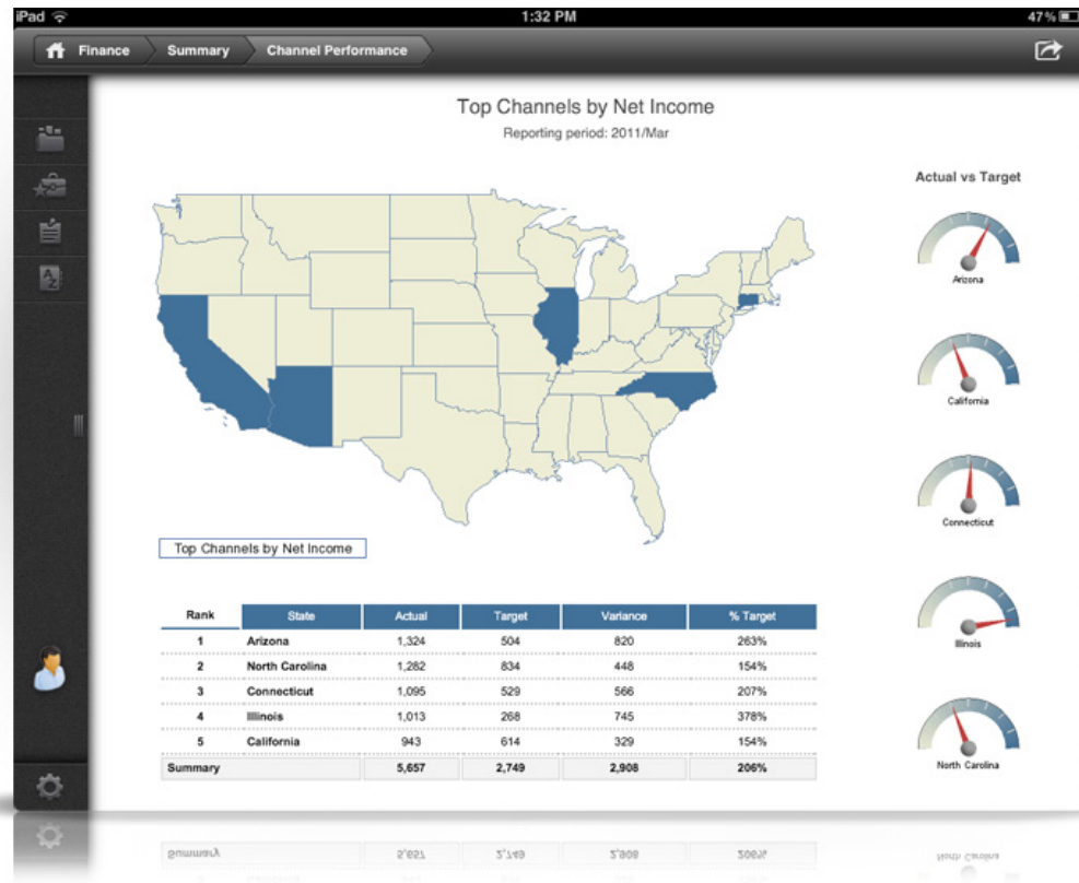
Intuitive Interface
