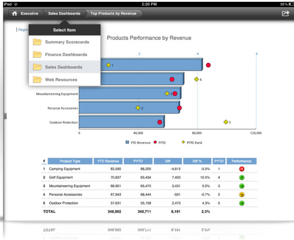
Breadcrumb Navigation
