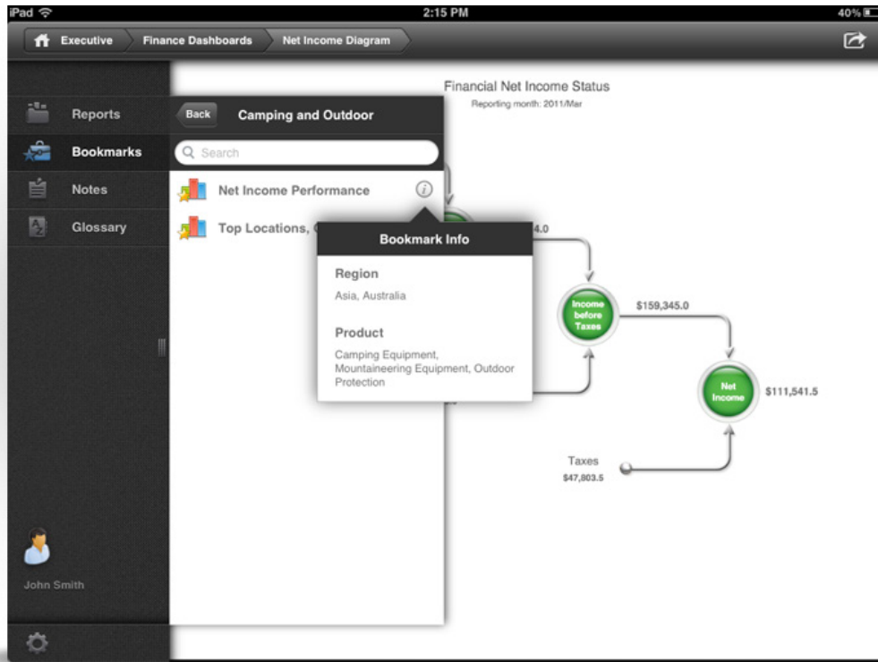
Bookmarks Panel
